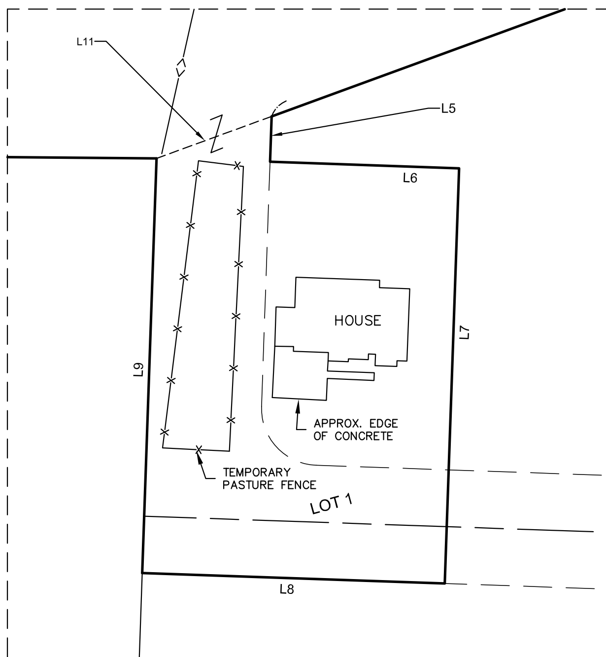
DETAIL - LOT 1 1"=50'
